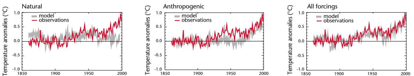
Figure 15. Comparing simulations of the Earth's annual global mean surface temperatures with measurements can provide insight into the underlying causes of major changes; adding the calculated effects of human-induced and natural forcings mimics actual observations (IPCC, 2001)
