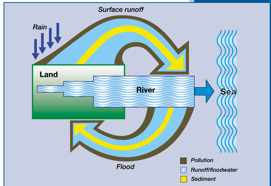
Figure 5. Schematic diagram of rainfall-induced processes involved in land degradation.
