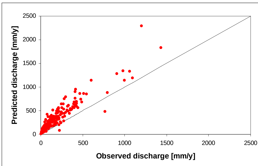
Figure 18: Comparison of CableDyn predictions and observations of discharge for 200 gauged catchments across Australia, averaged over the period (1/1/1981 to 31/12/2005).
