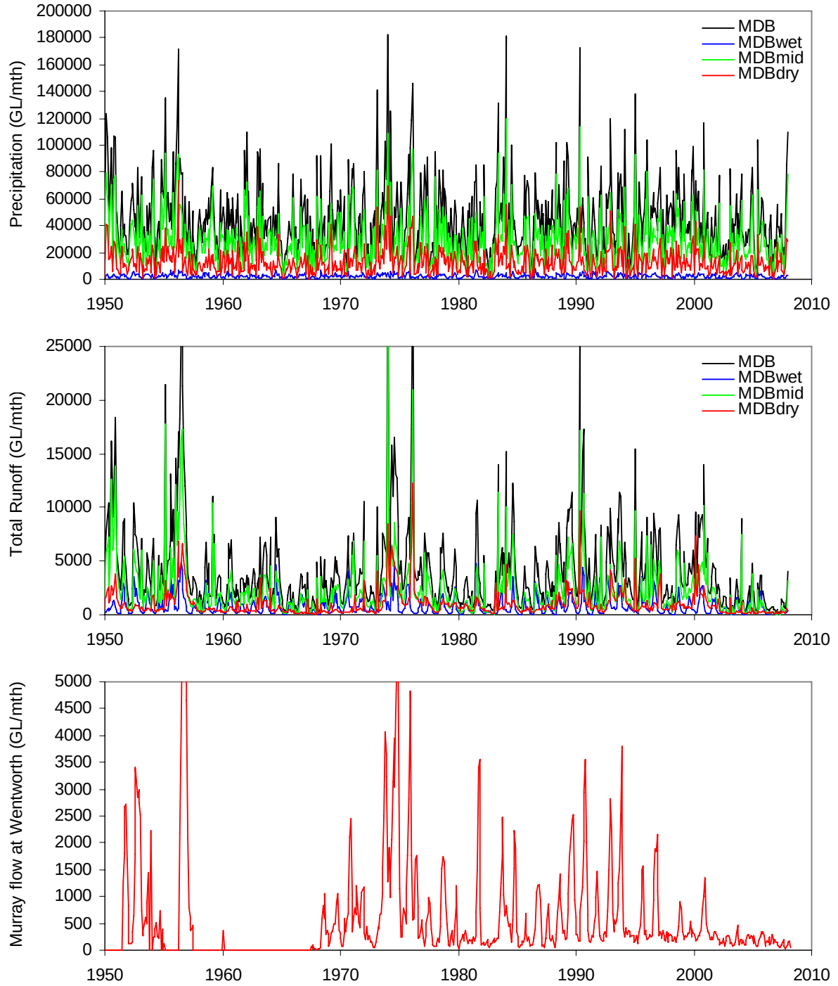
Figure 12: (top) monthly series of total precipitation ( P_{Land} ) falling on the MDB (black), with contributions falling on wet (blue), agricultural (green) and semi-arid (red) ANRA drainage basins in the MDB; (middle) total runoff ( R_{Land} ) from all land surfaces in the MDB (black), with contributions from wet (blue), agricultural (green) and semi-arid (red) drainage basins; (bottom) gauged flow in the Murray River at Wentworth ( Q_{River} ).
