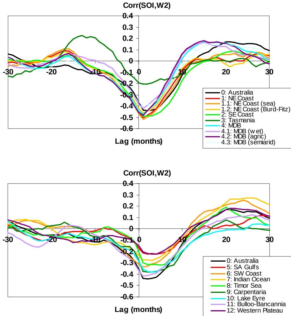
Figure 16: Lagged correlation between monthly SOI and lower-layer soil moisture averaged over Drainage Divisions in the eastern part of Australia (colours in upper panel) and the western part (colours in lower panel). Black lines in both panels are for lower-layer soil moisture averaged over the whole continent. Time period: 1955 to 2006. Model version and run: WaterDyn18M, Australia18a (using SILO meteorology).
