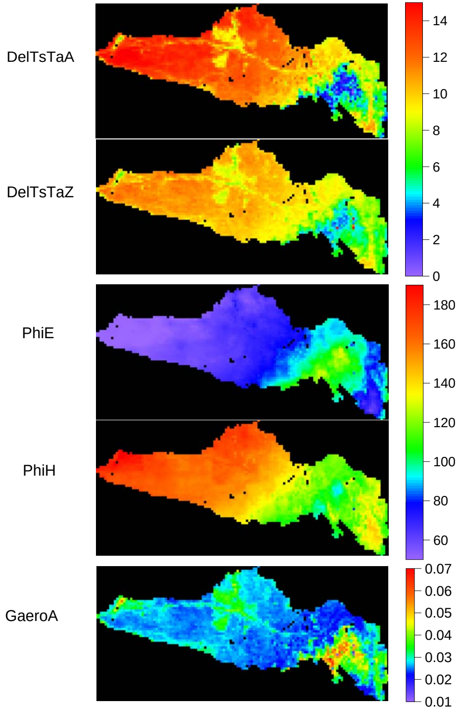
Figure 17: Illustration of determination of aerodynamic conductance G_a . First and second panels: observed and modelled surface-air temperature difference ( T_s - T_a , degC) in the Murrumbidgee basin. Third and fourth panels: modelled latent heat flux ( \Phi_E , \text{W m}^{-2} ) and sensible heat flux ( \Phi_H , \text{W m}^{-2} ). Bottom panel: estimated long-term aerodynamic conductance ( G_a , \text{m s}^{-1} ) from Equation (M12). All quantities are long-term averages over period of available LST observations (1992 to 2006). Run: Murrumbidgee24b.
