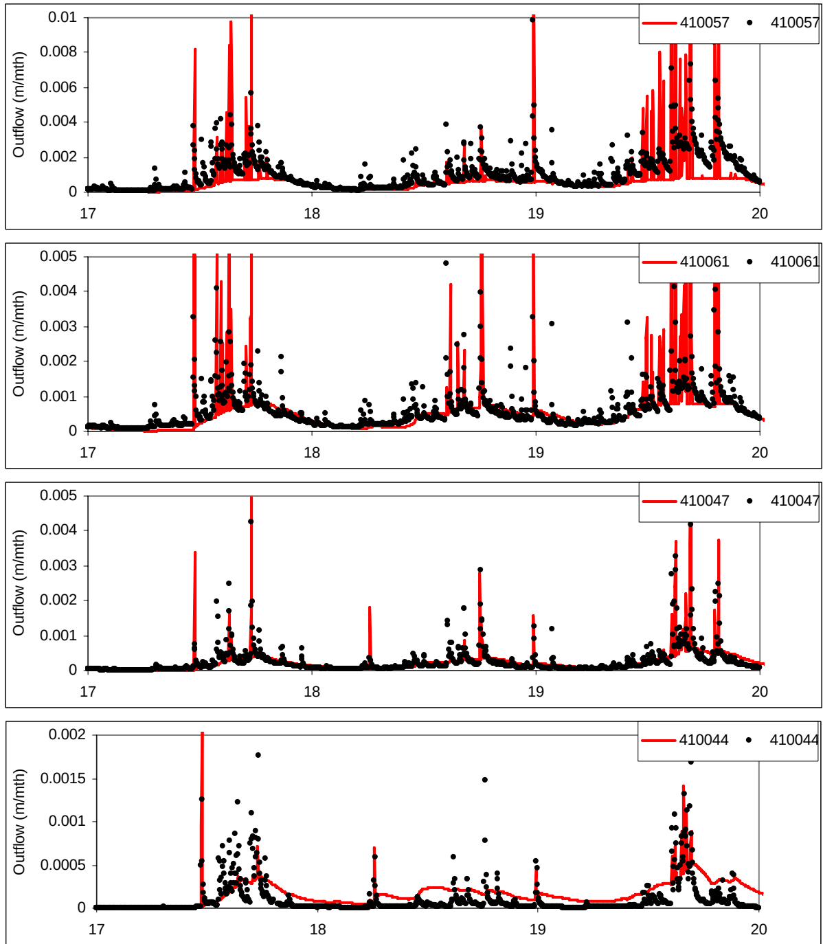
Figure 8b: As for Figure 8a, for daily outflow over 3 years. Time axis (17 to 20 years) runs from 1-jan-1998 to 31-dec-2000.
