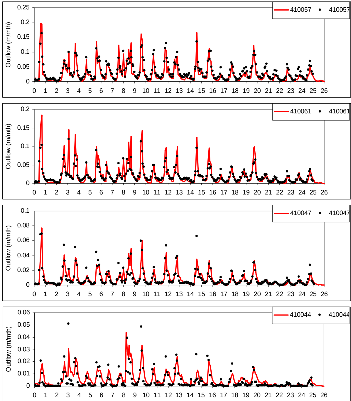
Figure 8a: Comparison of predicted (lines) and observed (points) monthly mean outflow for four unimpaired gauged catchments in the Murrumbidgee basin: Goobarragandra River at Lacmalac (410057), Adelong Creek at Batlow Road (410061), Tarcutta Creek at Old Borambola (410047) and Muttama Creek at Coolac (410044). Time axis (0 to 26 years) runs from 1-jan-1981 to 31-dec-2006. Model version and run: WaterDyn25M, Murrumbidgee25b2.
