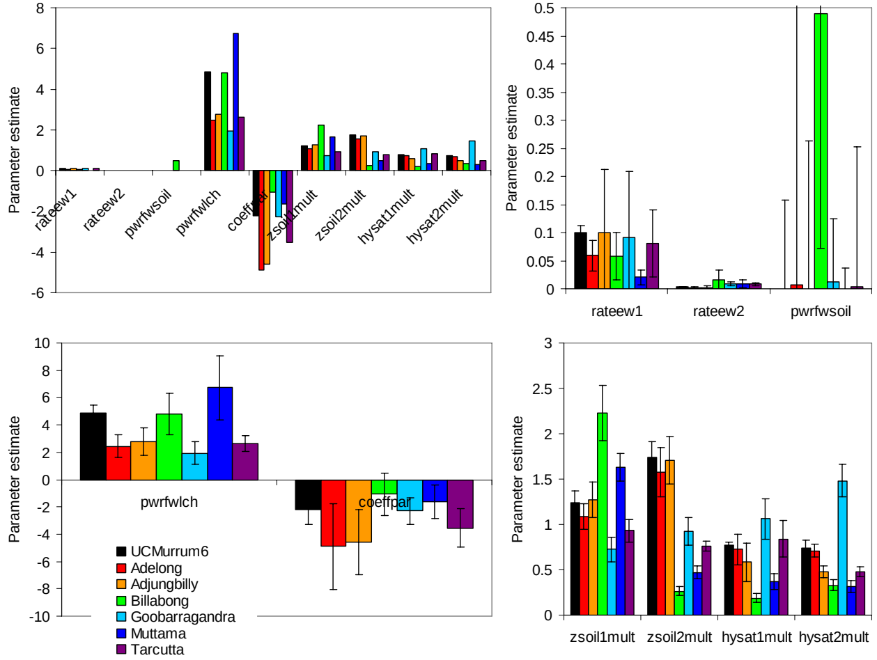
Figure 4: Estimates of 9 parameters (RateEW1, RateEW2, PwrFWSoil, PwrFWLch, CoeffPAR, ZSoil1Mult, ZSoil2Mult, HySat1Mult, HySat2Mult) = (k_{E1}, k_{E2}, \beta, \gamma, c_{PAR}, m_{Z1}, m_{Z2}, m_{K1}, m_{K2}) in 6 individual unimpaired catchments (coloured bars), and in all 6 catchments taken in aggregate (UCMurru6, black bars). Top left panel shows estimates of all 9 parameters on the same scale; other panels show groups of parameters on suitably expanded scales. Parameter estimation is by the down-gradient Levenberg-Marquardt (LM) method implemented in the PEST software package ( http://www.sspa.com/PEST/ ). Error bars denote 95% confidence intervals. Run: UCMurru25 (PEST mode).
