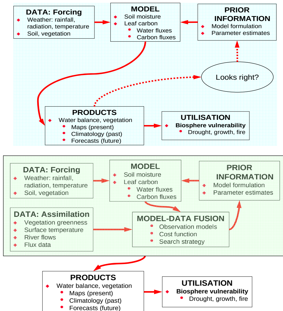
Figure 1: Schematic representation of components of a terrestrial-biosphere data assimilation system. Upper panel: without data assimilation; lower panel: with data assimilation.
