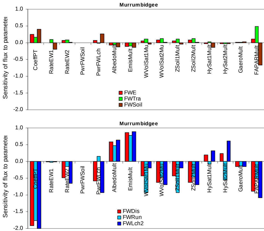
Figure 6b: Sensitivities of fluxes to parameters for the Murrumbidgee basin, with other details as for Figure 6a. Run: Murrumbidgee25b2.
