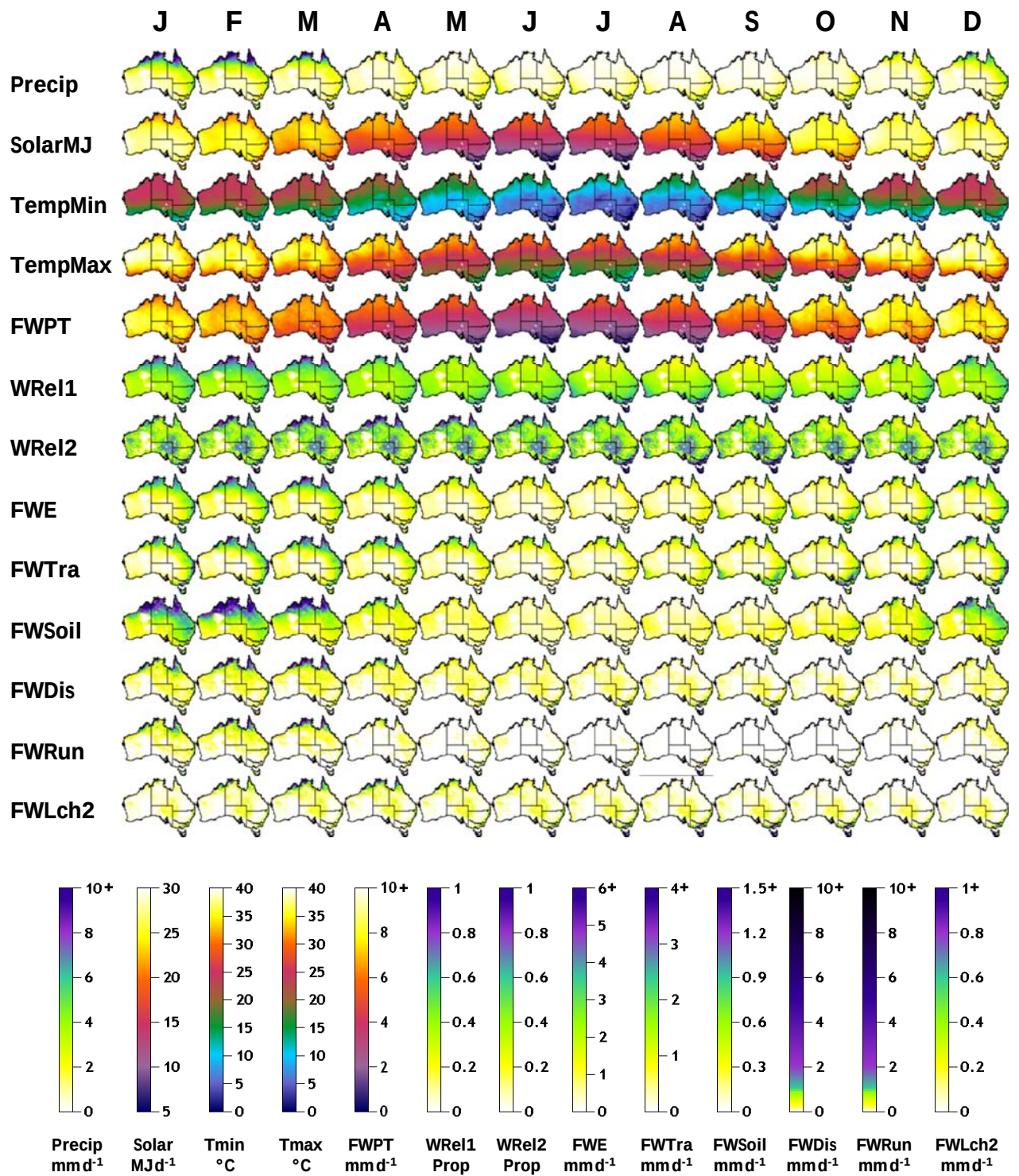
Figure 10: Australian monthly climatologies (reference period 1961-1990), except for solar irradiance (1990-2007). Variables: precipitation (Precip); solar irradiance (Solar); daily maximum and minimum air temperatures (Tmax, Tmin); Priestley-Taylor potential evaporation (FWPT); upper-layer and lower-layer relative water contents (WRel1, WRel2); total evapotranspiration (FWE); transpiration (FWTra), soil evaporation (FWSoil), total runoff (FWDIs); surface runoff (FWRUn), deep drainage (FWLch2). Model version and run: WaterDyn25M, Australia25a.
