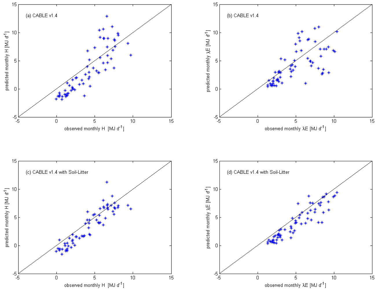
Figure 20: Comparisons of predicted and observed monthly mean H and \lambda E for simulations using CABLE v1.4 (a) and (b) and CABLE v1.4 with “Soil-Litter” (c) and (d).
