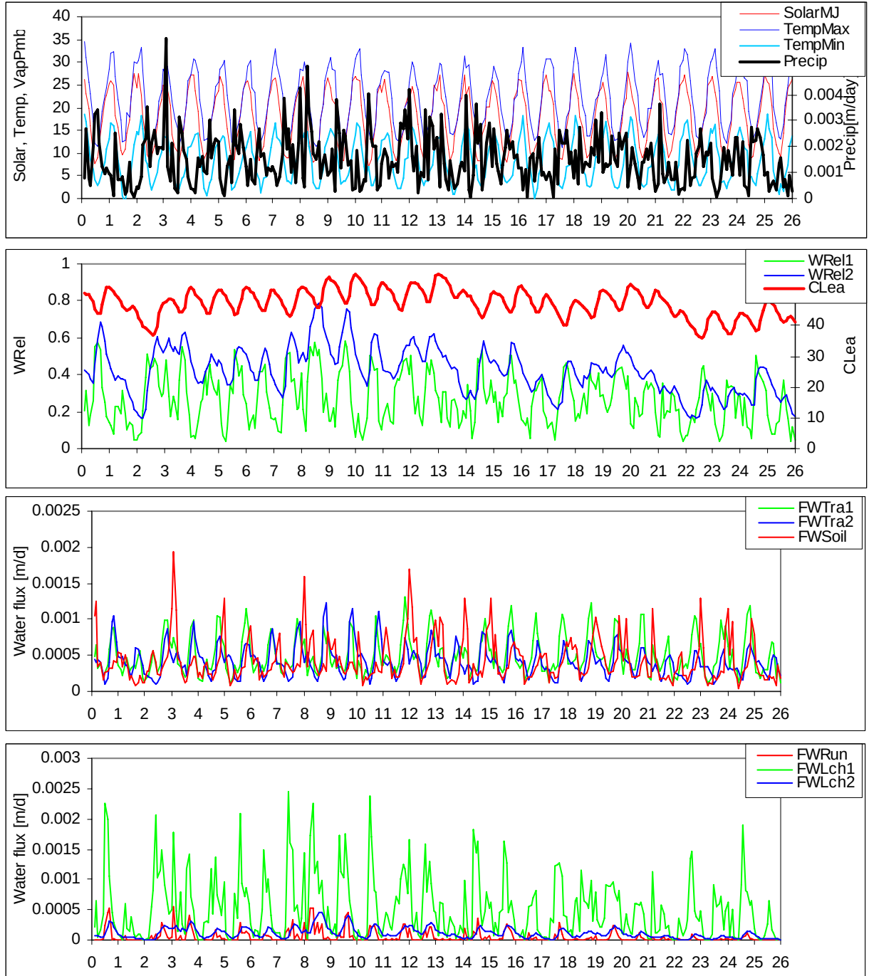
Figure 2: Spatially averaged monthly time series of WaterDyn inputs and selected outputs over the Murrumbidgee catchment. Time axis (0 to 26 years) runs from 1-jan-1981 to 31-dec-2006. Top panel: meteorological forcing, including precipitation, solar irradiance and daily maximum and minimum air temperatures; second panel: computed state variables, consisting of relative soil moisture in two layers ( w_{1,2} ) and green-leaf carbon store C_L ( \text{molC m}^{-2} ) (note that the computed store C_L is not used for water balance calculations); third panel: water fluxes contributing to evapotranspiration (including transpiration from upper and lower soil layers and soil evaporation); fourth panel: fluxes contributing to total runoff (including surface runoff, drainage from layer 1 to layer 2, deep drainage out of layer 2). Model version and run: WaterDyn25M, Murrumbidgee25b2.
