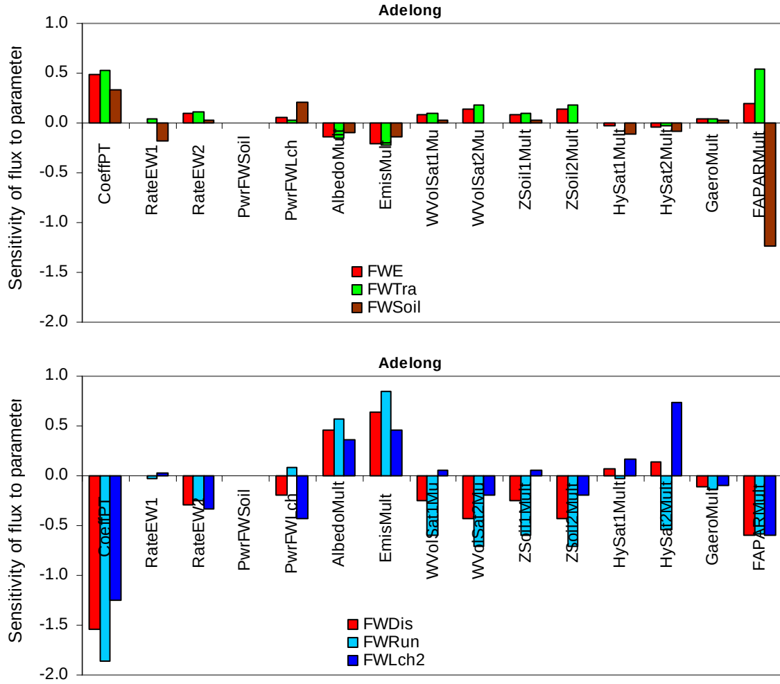
Figure 6a: Sensitivities of fluxes to parameters for the Adelong Creek catchment. Upper panel: total evapotranspiration ( F_{WE} = F_{WTra} + F_{WSoil} ) and its components, transpiration ( F_{WTra} ) and soil evaporation ( F_{WSoil} ). Lower panel: total runoff ( F_{WDis} = F_{WRun} + F_{WLch2} ) and its components, surface runoff ( F_{WRun} ) and deep drainage ( F_{WLch2} ). See Table C1 for parameter code names. Run: Adelong25b.
