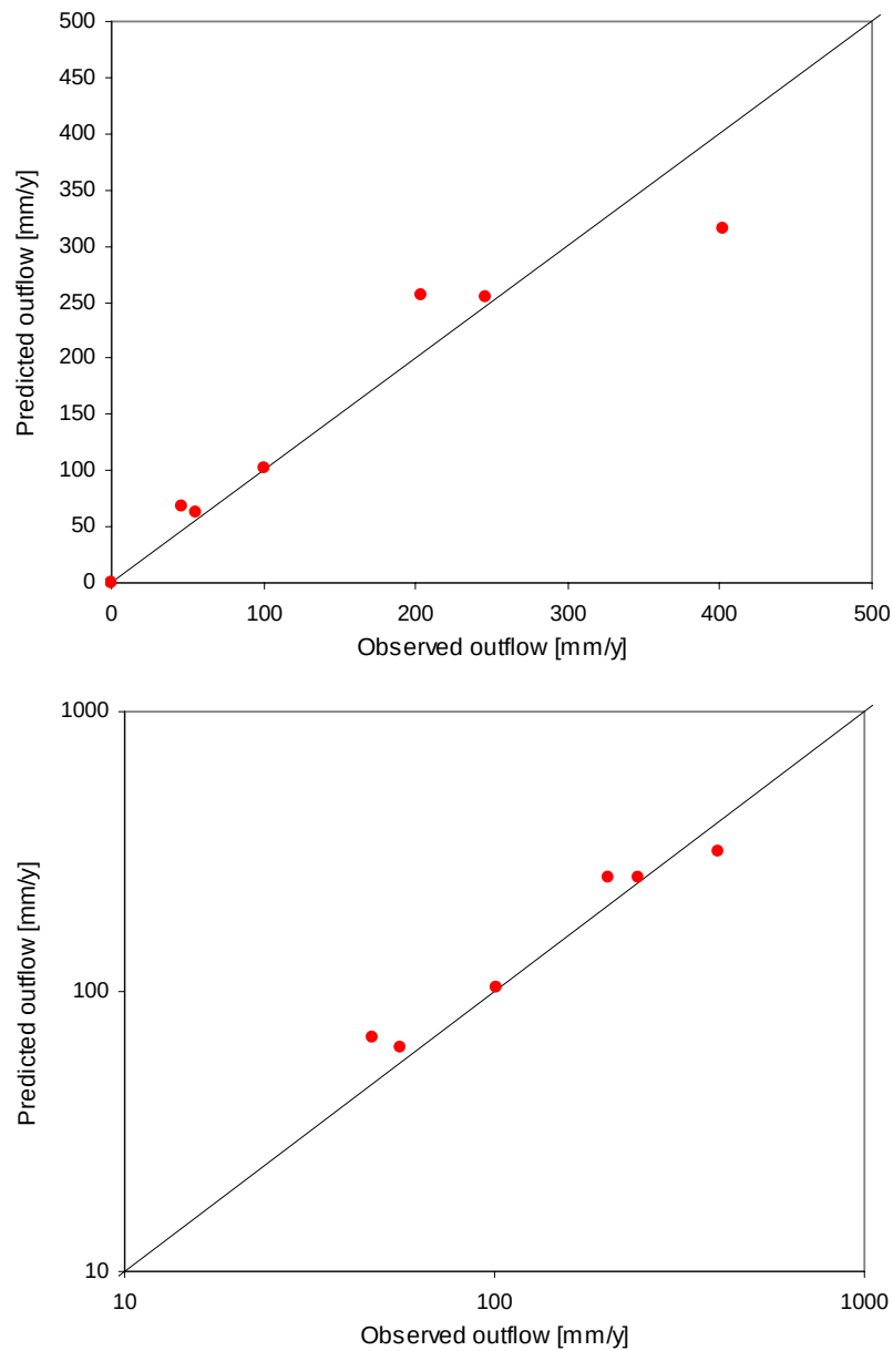
Figure 5: Predicted versus observed mean outflow (over available observations from 1981 to 2006 inclusive) for six nominally unimpaired gauged catchments in the Murrumbidgee basin (Table 1). Upper and lower panels use linear and logarithmic axes, respectively. Model version and run: WaterDyn25M, Murrumbidgee25b2.
