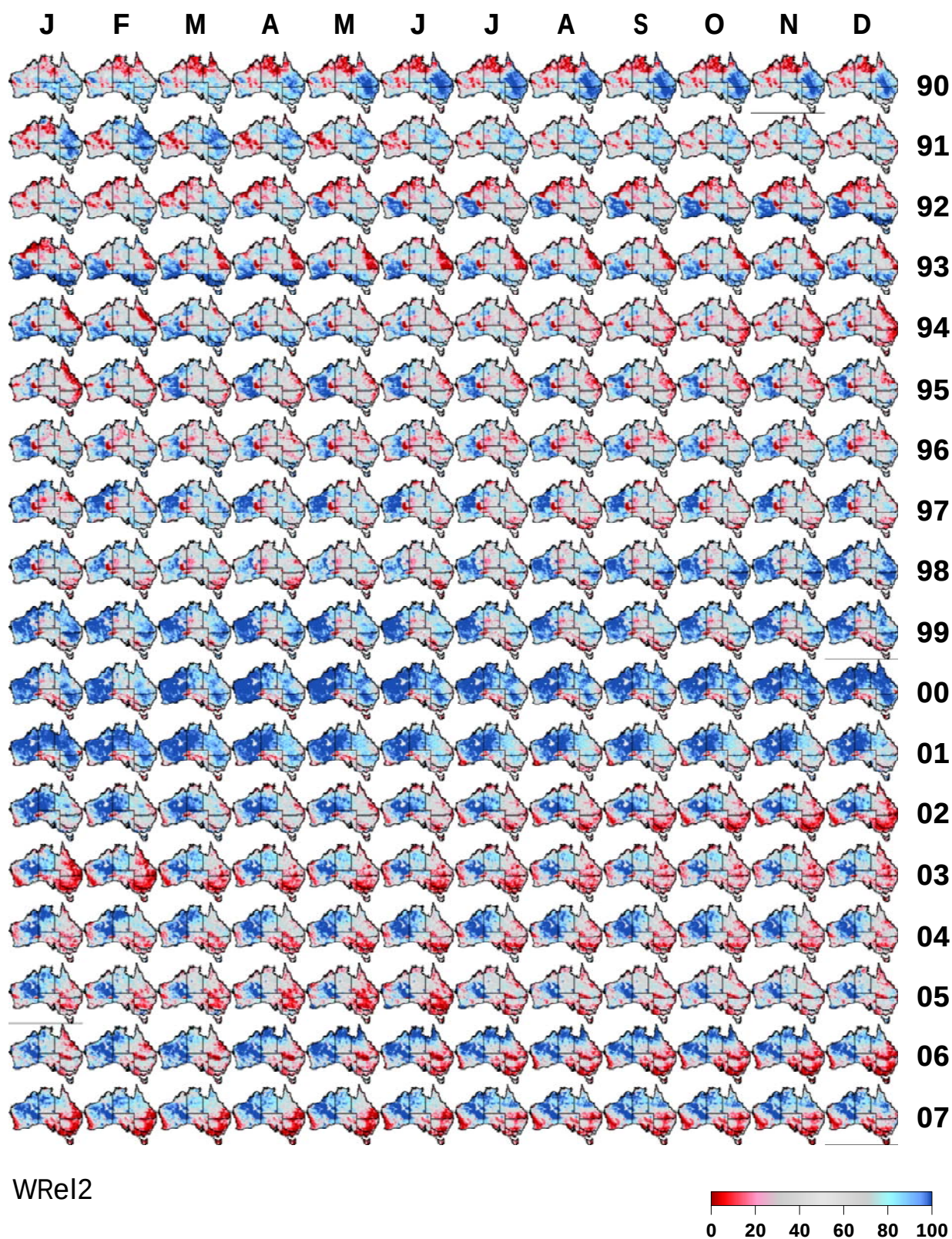
Figure 9b: As for Figure 9a, for monthly lower-layer relative soil moisture ( w_2 ).
