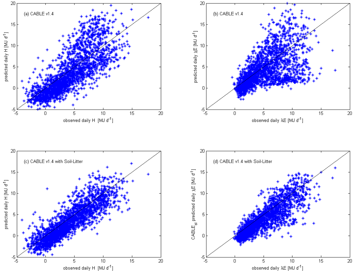
Figure 19: Comparisons of predicted and observed daily H and \lambda E for simulations using CABLE v1.4 (a) and (b) and CABLE v1.4 with “Soil-Litter” (c) and (d).
