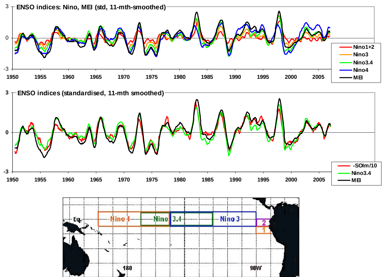
Figure 14: Time series of ENSO indices, detrended to second order and normalised to zero mean and unit variance. Top: Niño1+2 average (red), Niño3 (orange), Niño3.4 (green), Niño4 (blue), MEI (black). Middle: SOI (red), Niño3.4 (green), MEI (black). Bottom: location of ocean regions defining the Niño1, Niño2, Niño3, Niño3.4 and Niño4 sea surface temperatures. The Multivariate ENSO Index (MEI) constructed from the first principal components of sea-level pressure, zonal and meridional components of the surface wind, sea surface temperature, surface air temperature, and total sky cloudiness fraction (Wolter and Timlin 1993; Wolter and Timlin 1998). Monthly time series for Niño3, Niño3.4, Niño4 are from [http://www.cpc.ncep.noaa.gov/data/indices/sstoi.indices] . Series for the MEI are from [http://www.cdc.noaa.gov/ClimateIndices/List/] . Series for the SOI are from the Bureau of Meteorology [http://www.bom.gov.au/climate/current/soihtml1.shtml] with sign reversal and rescaling to match other indices.
