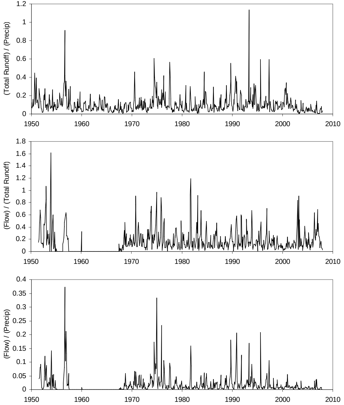
Figure 13: (top) transmission fraction f_{Land} = R_{Land}/P_{Land} ; (middle) transmission fraction f_{River} = Q_{River}/R_{Land} ; (bottom) total transmission fraction f_{Total} = f_{Land}f_{River} = Q_{River}/P_{Land} .
