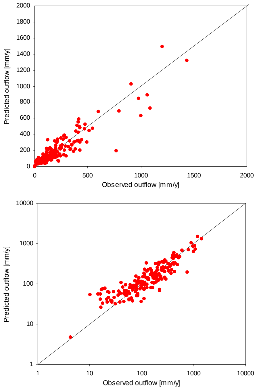
Figure 7: Predicted versus observed mean outflow (over available observations from 1981 to 2006 inclusive) for 200 unimpaired gauged catchments across Australia. Upper and lower panels use linear and logarithmic axes, respectively. Model version and run: WaterDyn25M, UCA1125b2.
