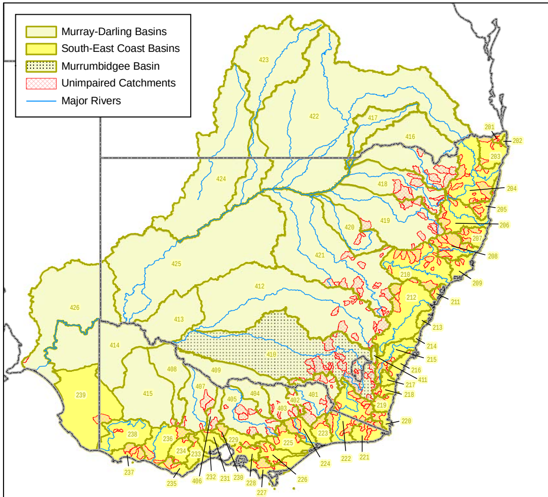
Figure 3: Nominally unimpaired catchments in southeast Australia (hatched red areas), superimposed on spatial domain maps for the Murray-Darling Basin (light olive) and South-East Coast Drainage Divisions as defined by the Australian National Resources Audit (ANRA) (NLWRA 2001a; NLWRA 2001b). The Murrumbidgee basin (410) is stippled in black.
