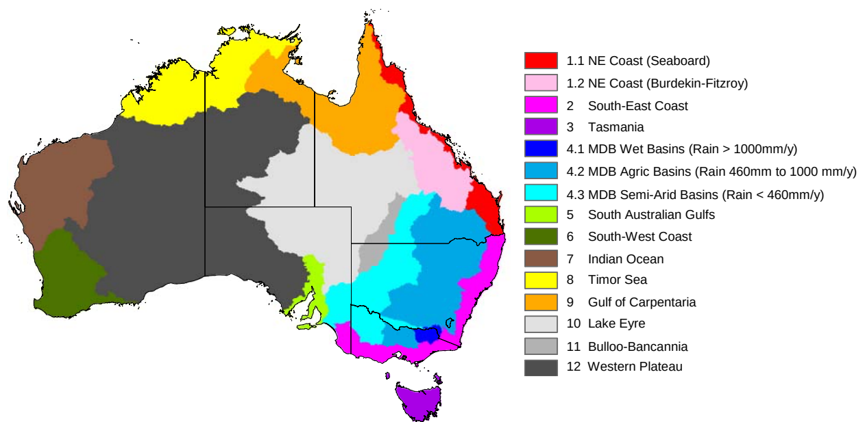
Figure 11: Regionalisation of the Australian continent into Australian National Resources Audit (ANRA) Drainage Divisions (NLWRA 2001a; NLWRA 2001b). There are 12 primary ANRA Drainage Divisions, each an aggregate of a number of Drainage Basins (see Figure 3 for examples). In the above regionalisation, two ANRA Divisions with highly diverse biogeography and hydroclimatology have been subdivided into parts which are still aggregates of Drainage Basins, as follows. The NE Coast (Division 1) has been divided into seaboard basins (denoted 1.1) and the Burdekin and Fitzroy basins (denoted 1.2) which are primarily inland and drier. The Murray-Darling Basin (Division 4) has been subdivided into wet, agricultural and semi-arid basins (respectively denoted 4.1, 4.2 and 4.3), where wet basins have mean annual rainfall exceeding 1000 \text{ mm y}^{-1} , semi-arid basins have rainfall less than 460 \text{ mm y}^{-1} , and agricultural basins fall between these points. The final regionalisation has 15 regions.
